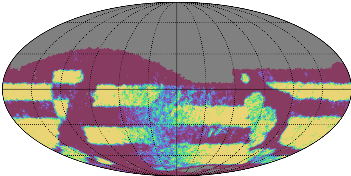
weather_cloudso1v3.4_10yrs Yr 3-4 r band: NVisits
