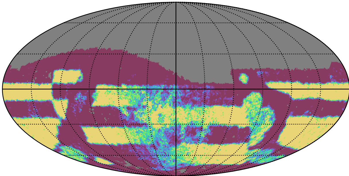
weather_cloudso1v3.4_10yrs Yr 3-4 i band: NVisits
