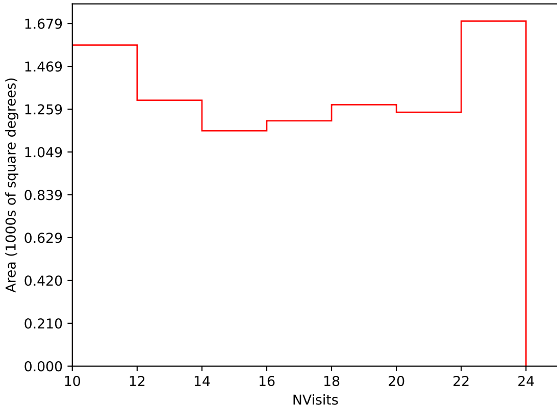
weather_cloudso1v3.4_10yrs Yr 3-4 i band: NVisits
