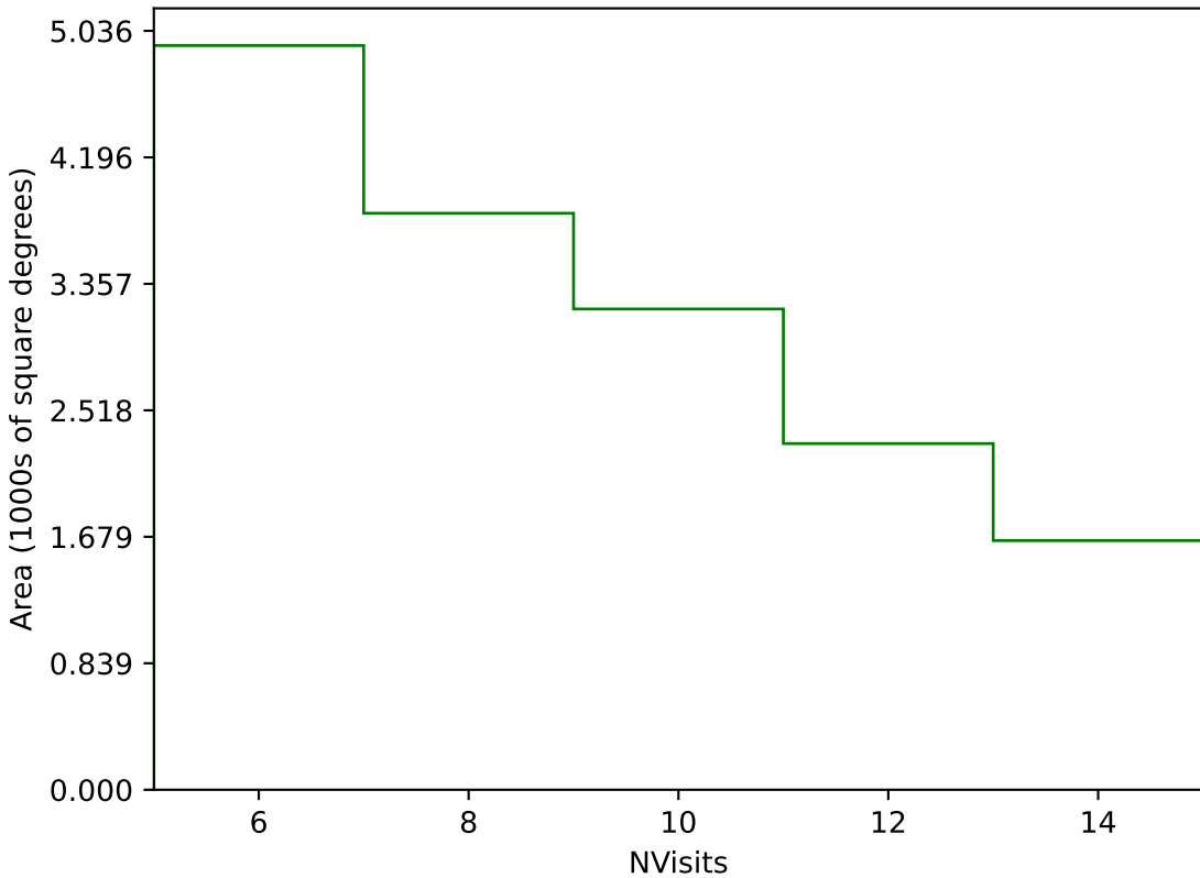
weather_cloudso1v3.4_10yrs Yr 3-4 g band: NVisits
