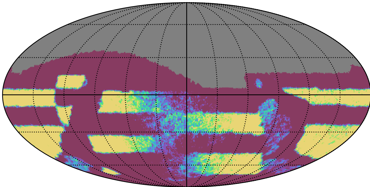
weather_cloudso1v3.4_10yrs Yr 3-4 all bands: NVisits
