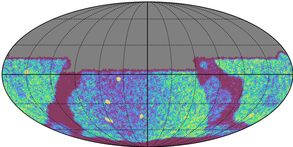
weather_cloudso1v3.4_10yrs Yr 1 y band: NVisits
