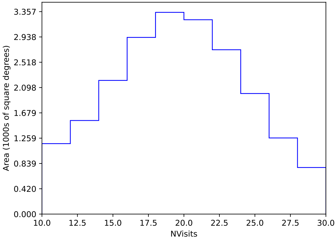
weather_cloudso1v3.4_10yrs Yr 1 y band: NVisits
