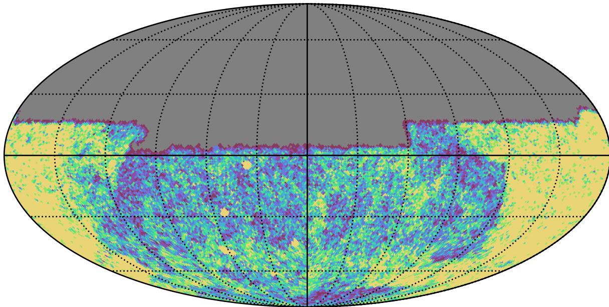
weather_cloudso1v3.4_10yrs Yr 1 u band: NVisits
