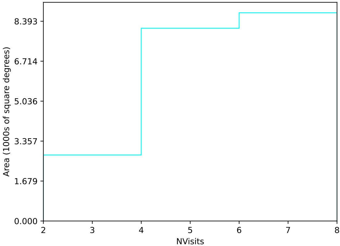
weather_cloudso1v3.4_10yrs Yr 1 u band: NVisits
