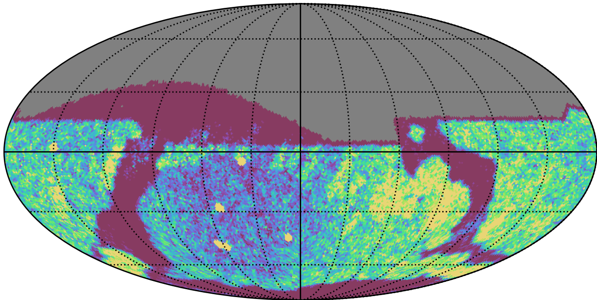
weather_cloudso1v3.4_10yrs Yr 1 r band: NVisits
