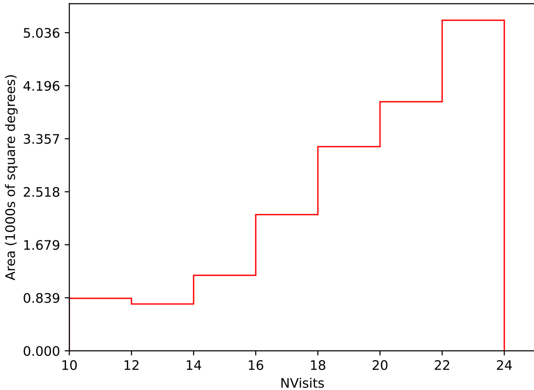
weather_cloudso1v3.4_10yrs Yr 1 i band: NVisits
