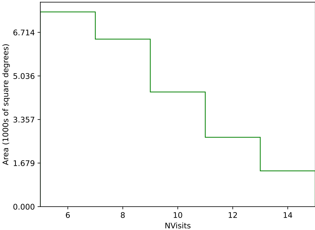
weather_cloudso1v3.4_10yrs Yr 1 g band: NVisits
