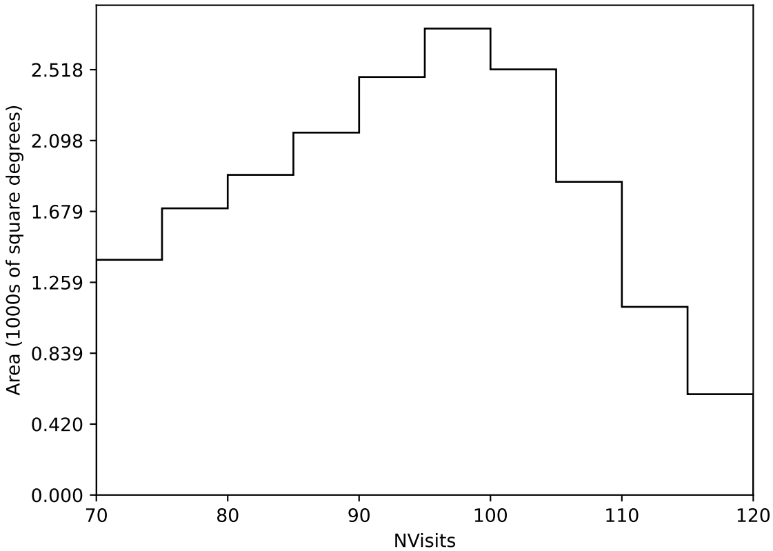
weather_cloudso1v3.4_10yrs Yr 1 all bands: NVisits
