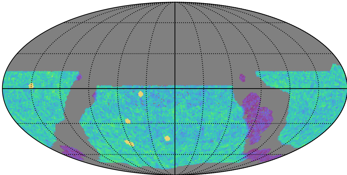
weather_cloudso1v3.4_10yrs WFD u band: NVisits
