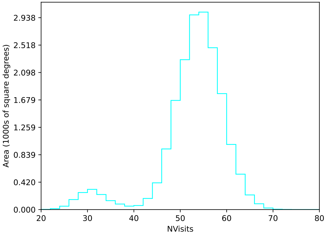
weather_cloudso1v3.4_10yrs WFD u band: NVisits
