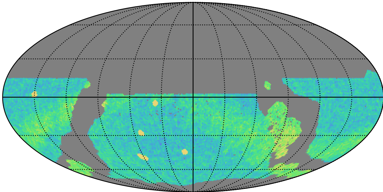
weather_cloudso1v3.4_10yrs WFD r band: NVisits
