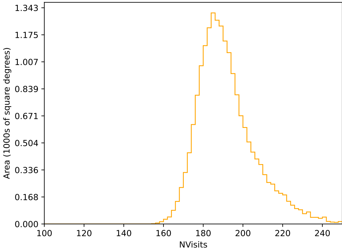
weather_cloudso1v3.4_10yrs WFD r band: NVisits
