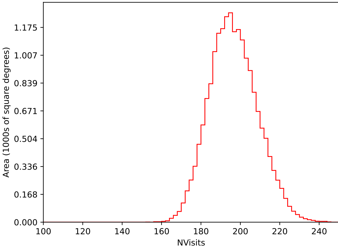
weather_cloudso1v3.4_10yrs WFD i band: NVisits
