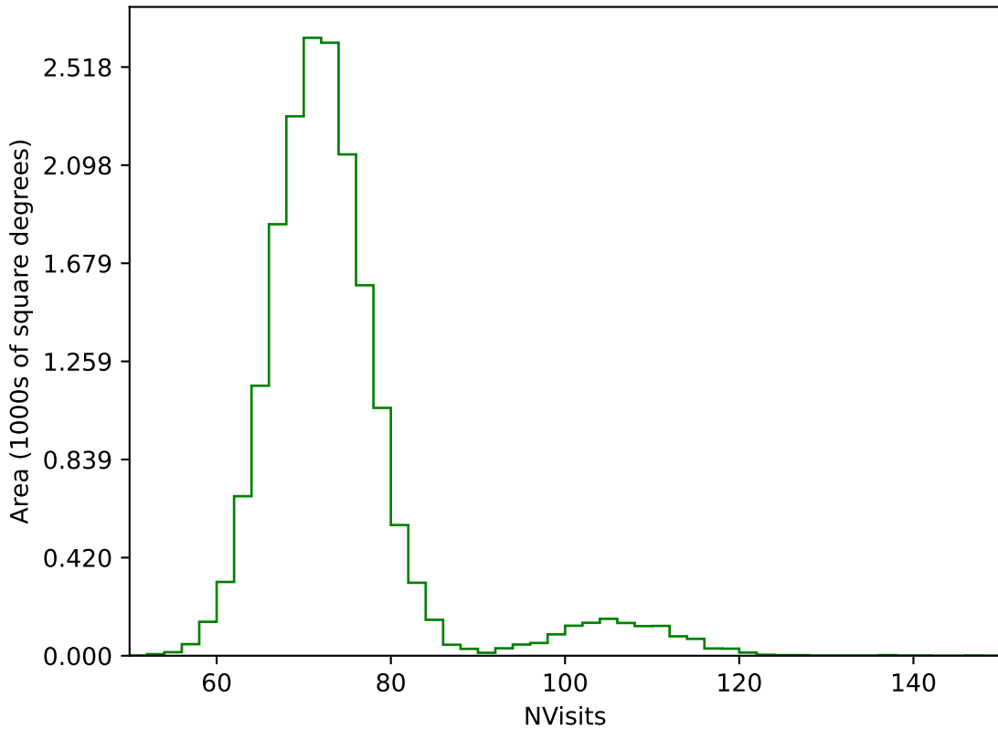
weather_cloudso1v3.4_10yrs WFD g band: NVisits
