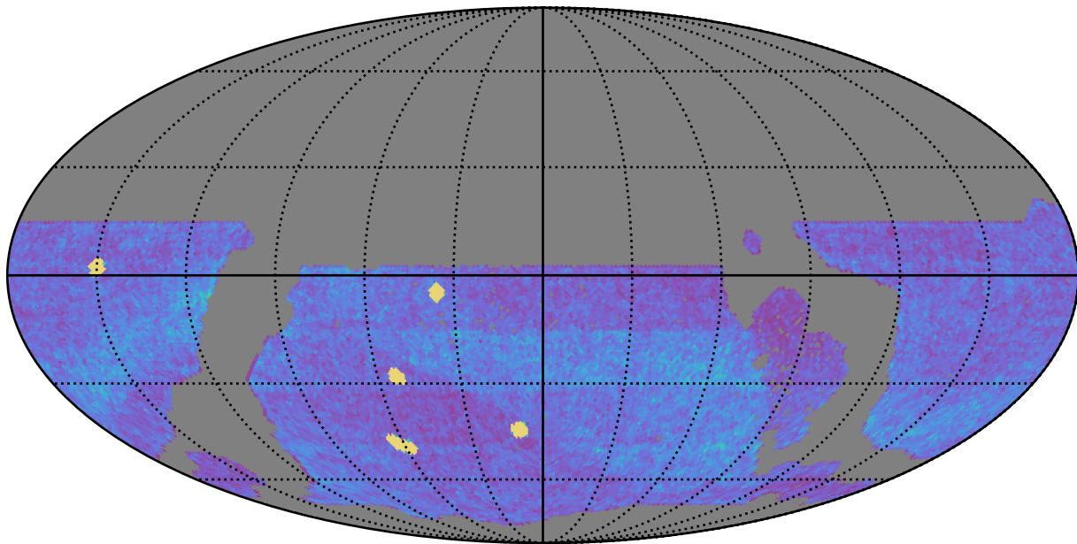
weather_cloudso1v3.4_10yrs WFD all bands: NVisits
