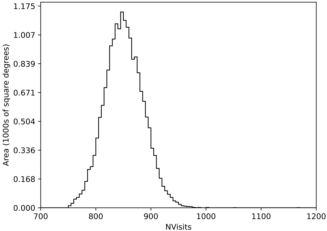
weather_cloudso1v3.4_10yrs WFD all bands: NVisits
