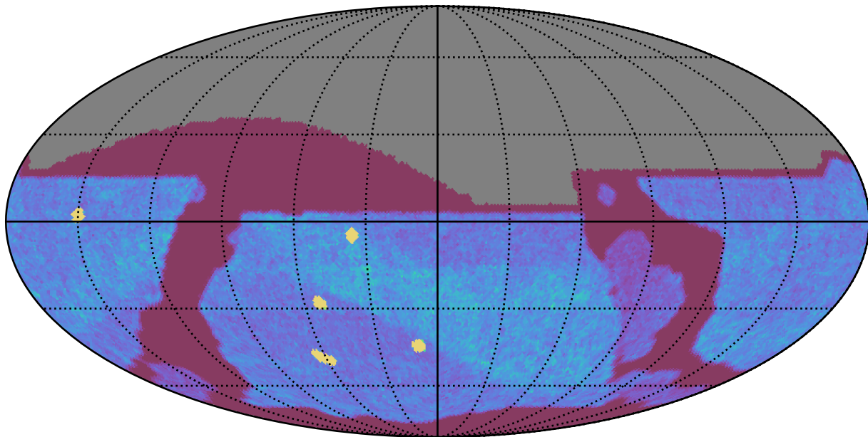
weather_cloudso1v3.4_10yrs All sky z band: NVisits
