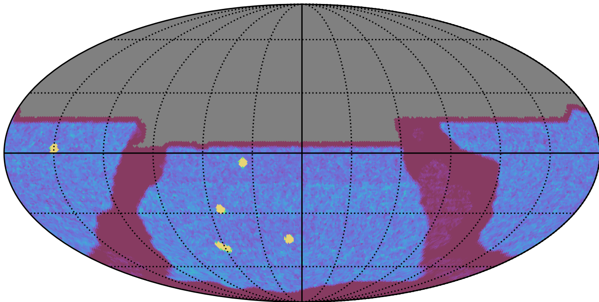
weather_cloudso1v3.4_10yrs All sky y band: NVisits
