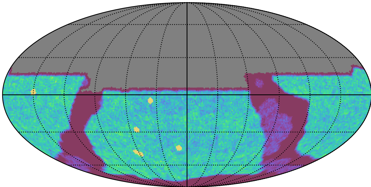
weather_cloudso1v3.4_10yrs All sky u band: NVisits
