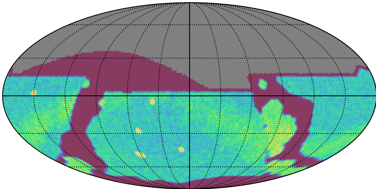
weather_cloudso1v3.4_10yrs All sky r band: NVisits
