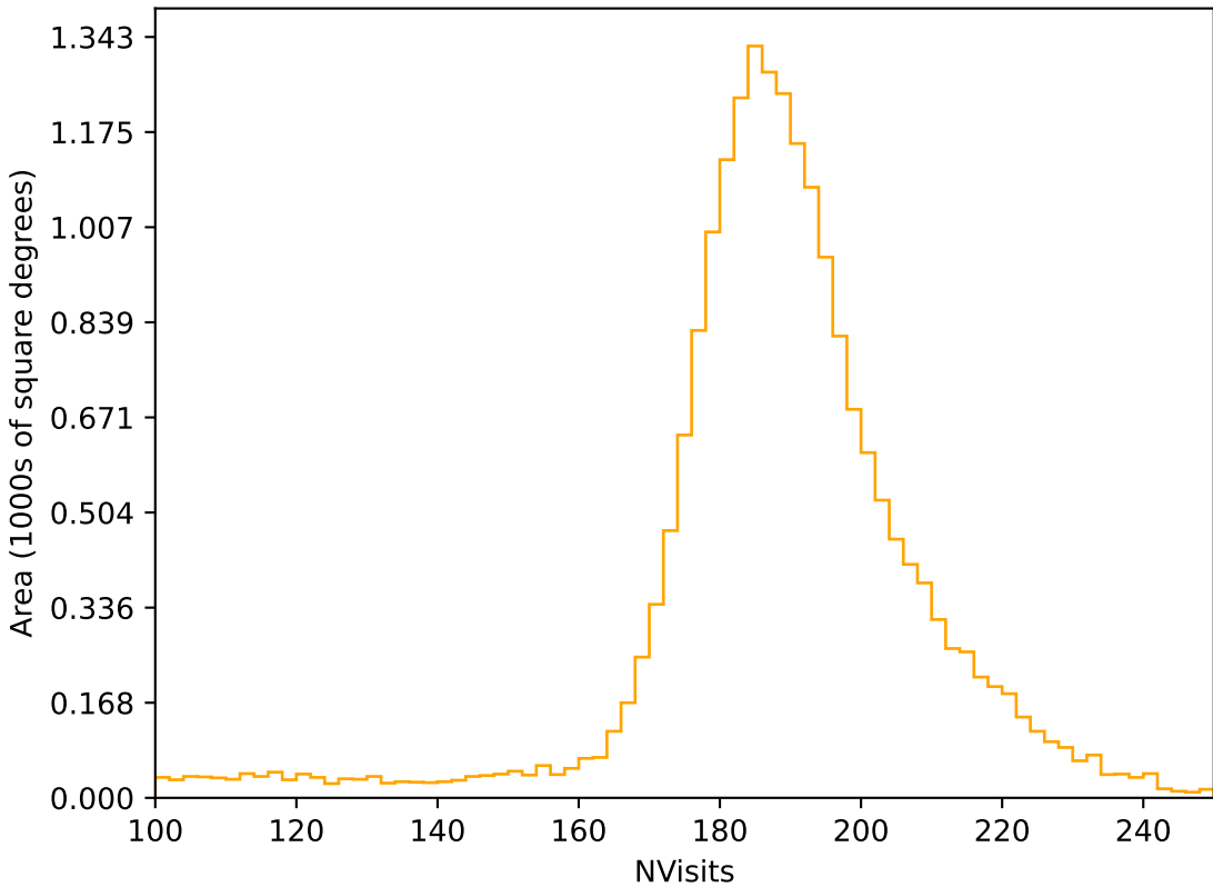
weather_cloudso1v3.4_10yrs All sky r band: NVisits
