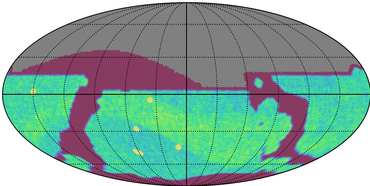
weather_cloudso1v3.4_10yrs All sky i band: NVisits
