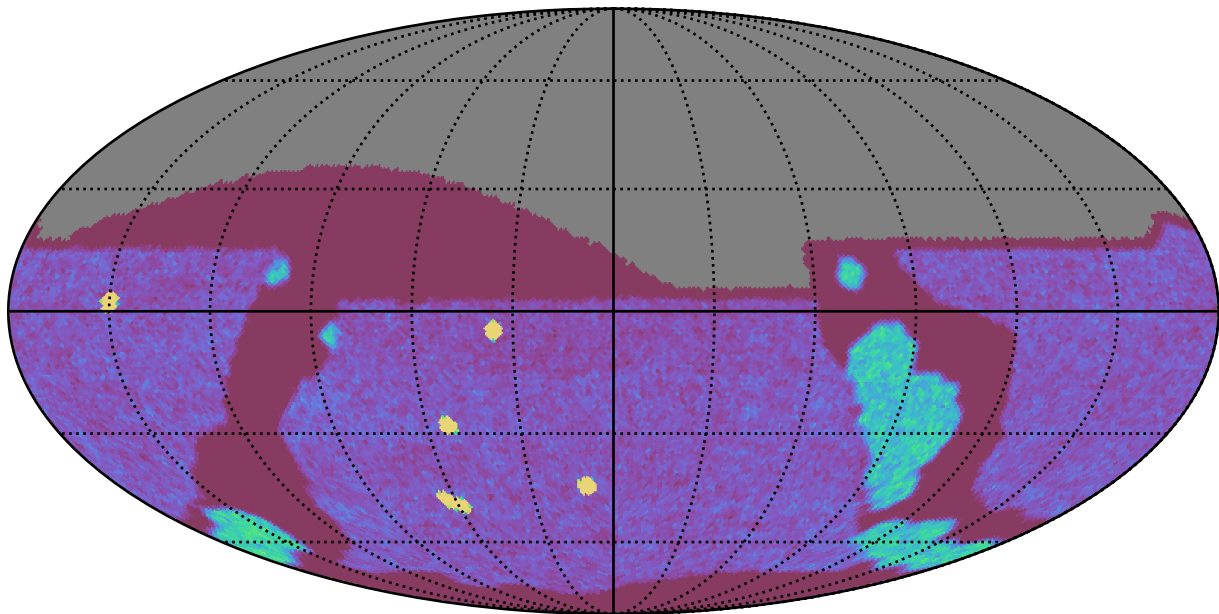
weather_cloudso1v3.4_10yrs All sky g band: NVisits
