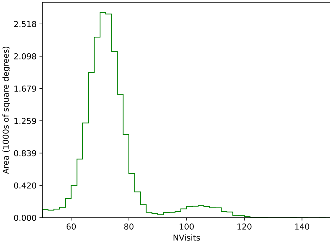
weather_cloudso1v3.4_10yrs All sky g band: NVisits
