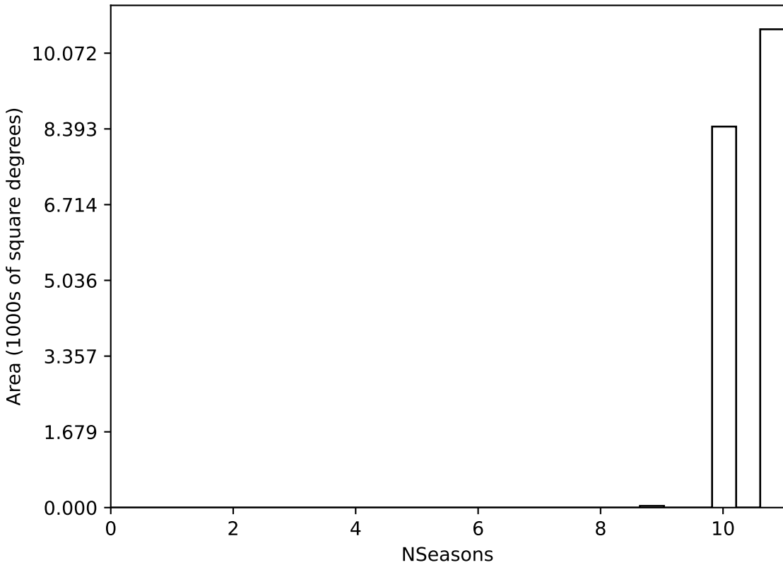
weather_cloudso1v3.4_10yrs WFD all bands: NSeasons
