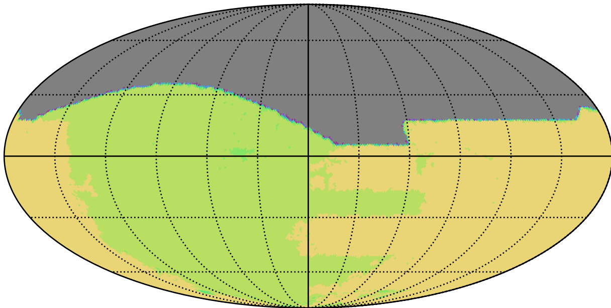
weather_cloudso1v3.4_10yrs All sky all bands: NSeasons
