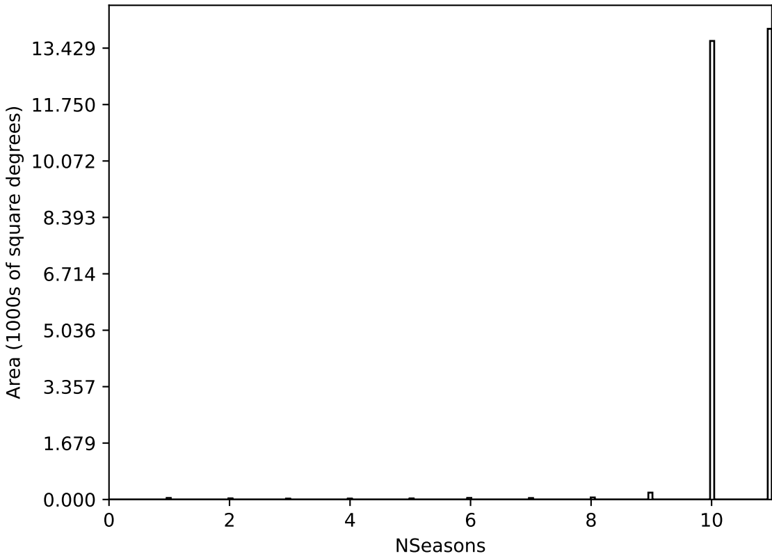
weather_cloudso1v3.4_10yrs All sky all bands: NSeasons
