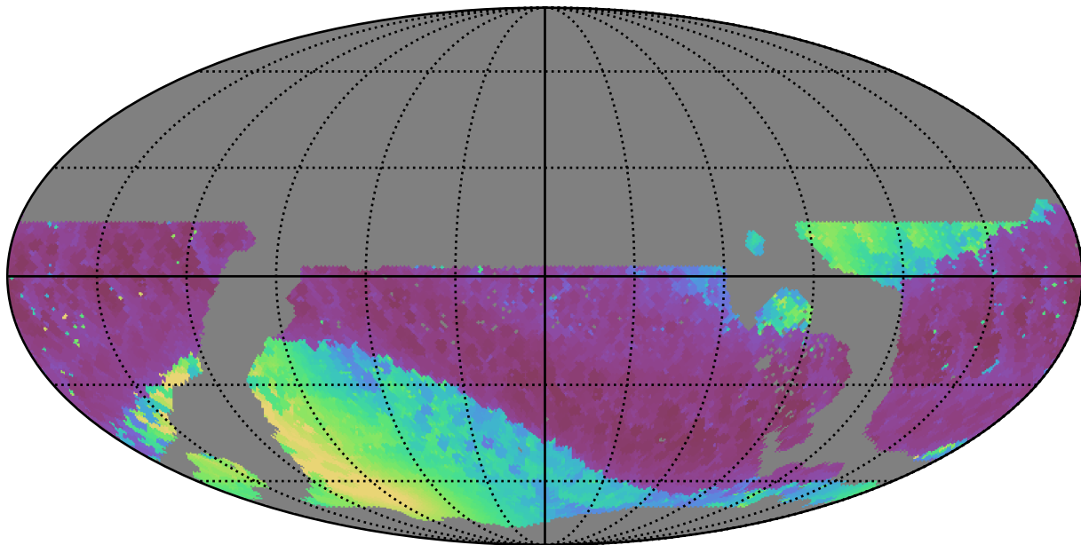
weather_cloudso1v3.4_10yrs WFD z band: Min solarElong
