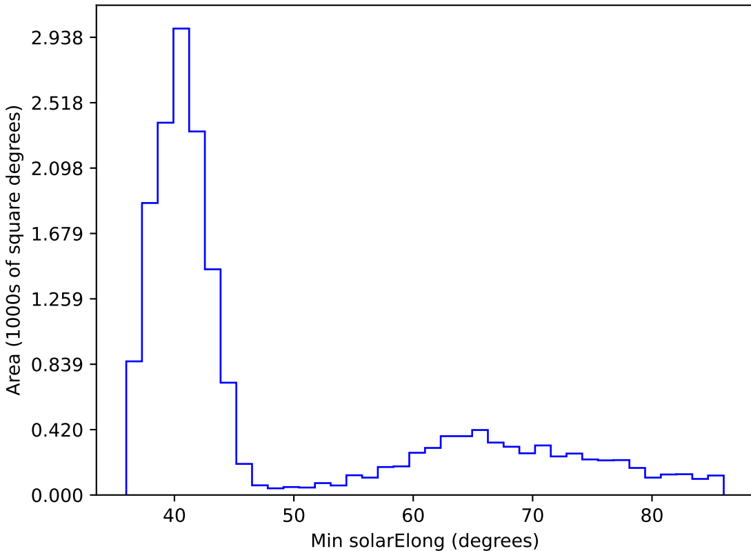
weather_cloudso1v3.4_10yrs WFD z band: Min solarElong
