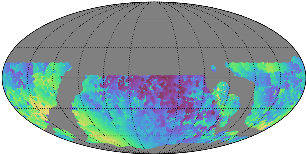
weather_cloudso1v3.4_10yrs WFD y band: Min solarElong
