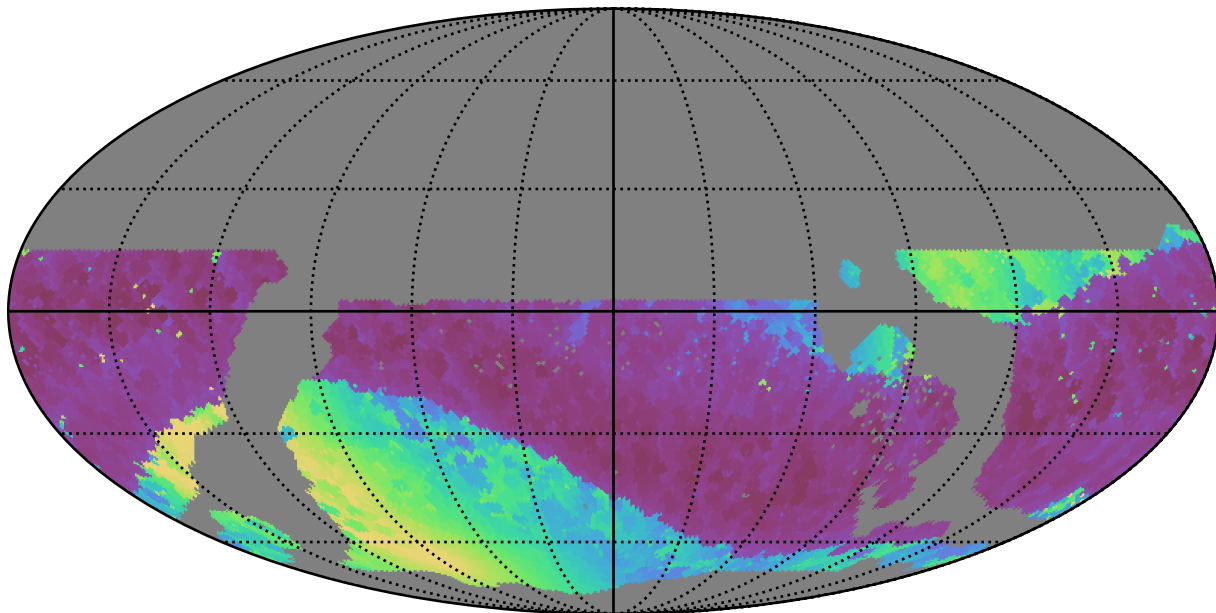
weather_cloudso1v3.4_10yrs WFD i band: Min solarElong
