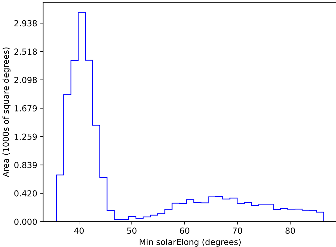
weather_cloudso1v3.4_10yrs WFD i band: Min solarElong
