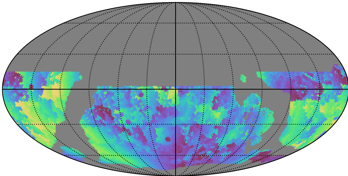
weather_cloudso1v3.4_10yrs WFD g band: Min solarElong
