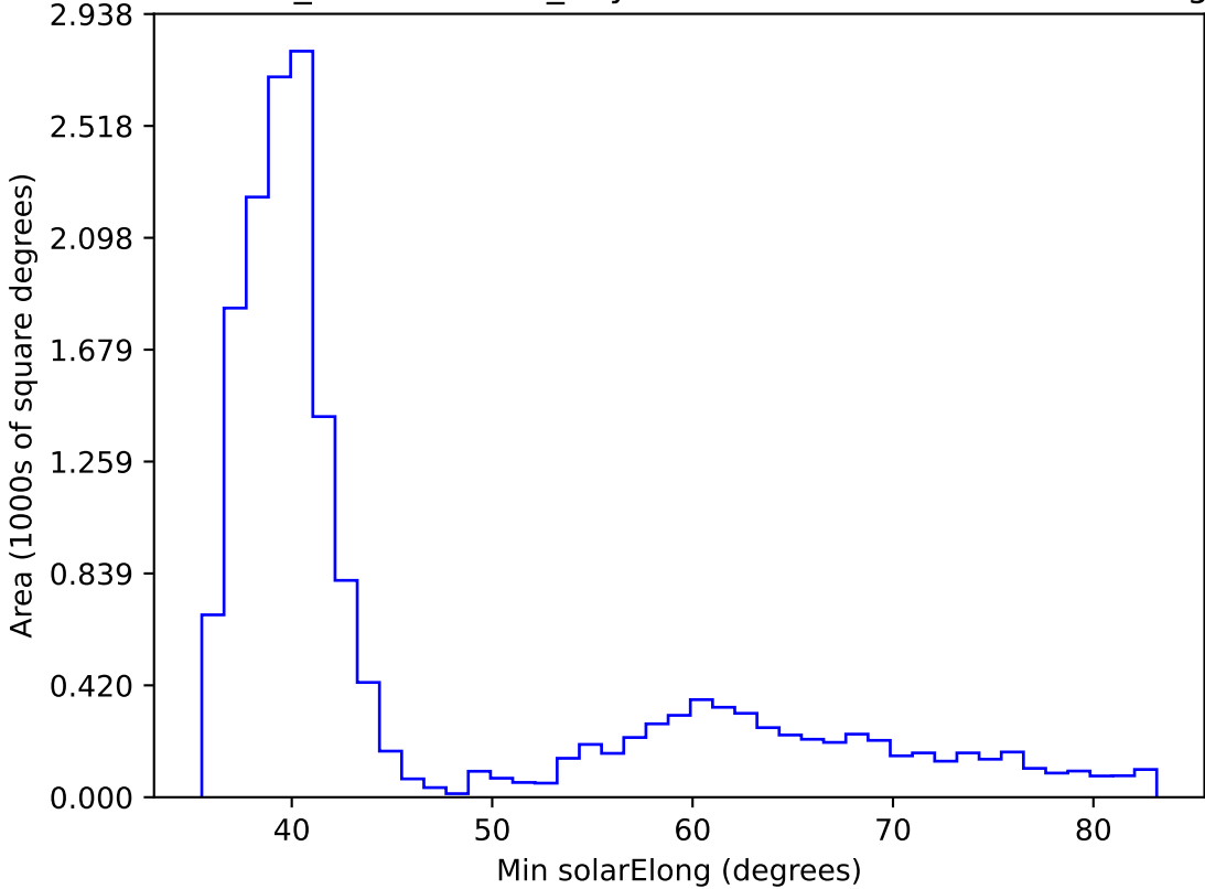
weather_cloudso1v3.4_10yrs WFD all bands: Min solarElong
