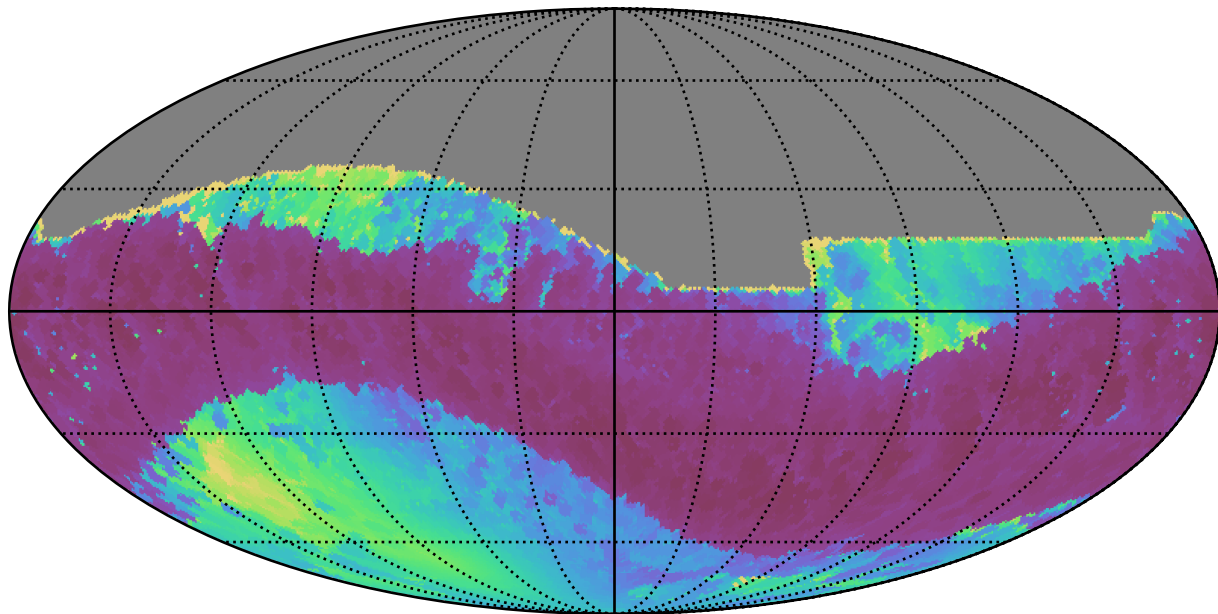
weather_cloudso1v3.4_10yrs All sky z band: Min solarElong
