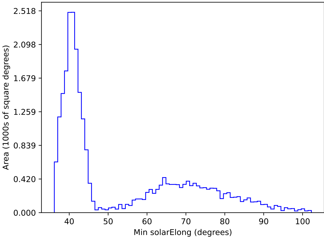
weather_cloudso1v3.4_10yrs All sky z band: Min solarElong
