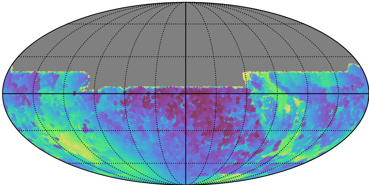
weather_cloudso1v3.4_10yrs All sky y band: Min solarElong
