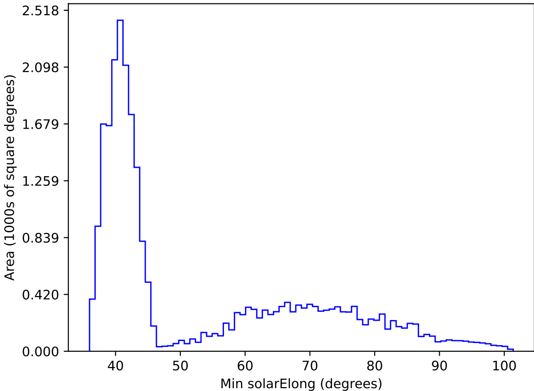
weather_cloudso1v3.4_10yrs All sky i band: Min solarElong
