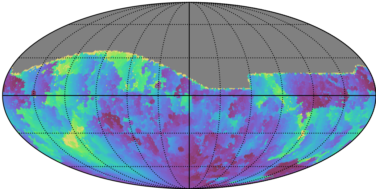
weather_cloudso1v3.4_10yrs All sky g band: Min solarElong
