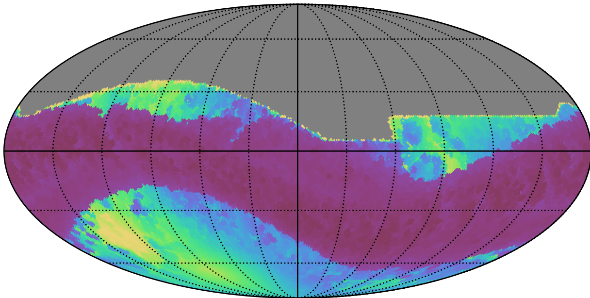
weather_cloudso1v3.4_10yrs All sky all bands: Min solarElong
