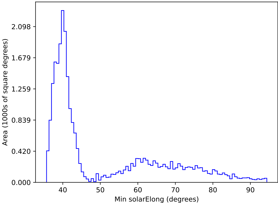
weather_cloudso1v3.4_10yrs All sky all bands: Min solarElong
