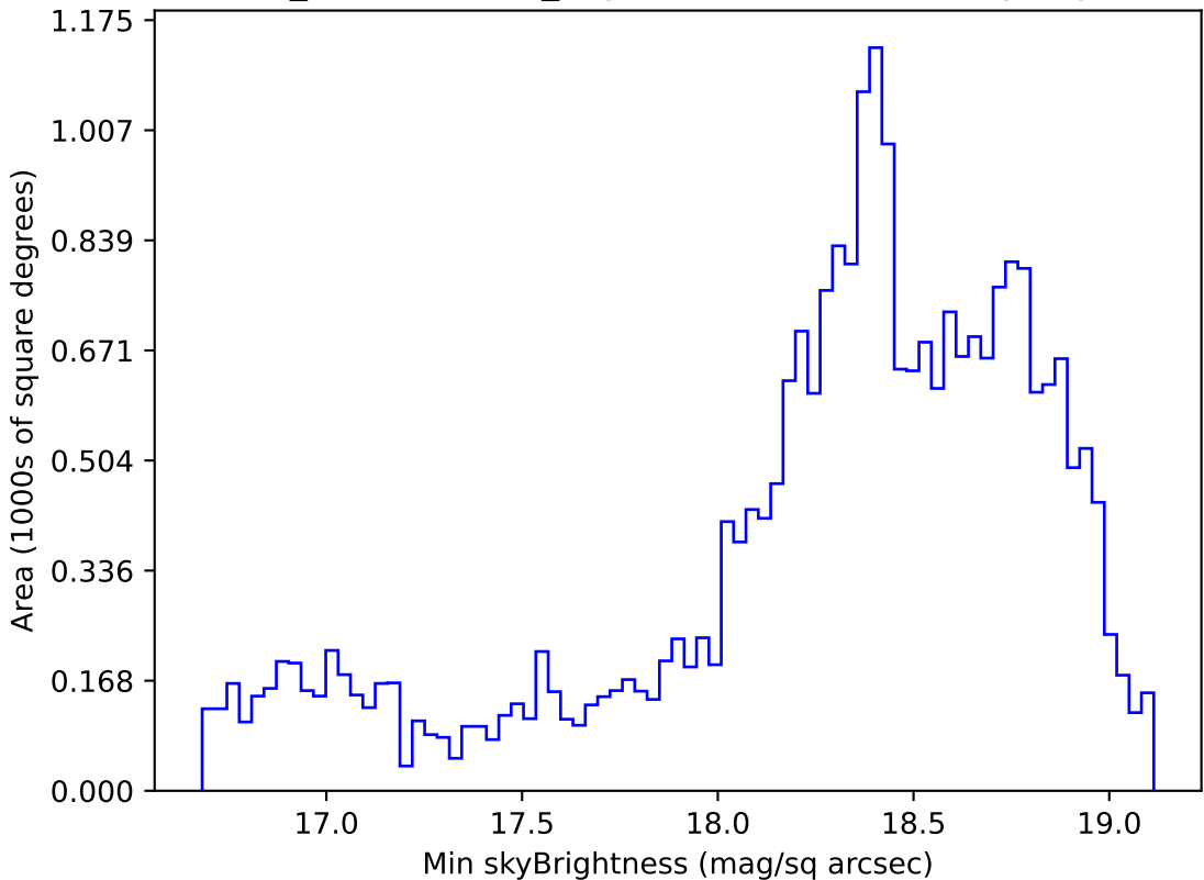
weather_cloudso1v3.4_10yrs Yr 1 z band: Min skyBrightness
