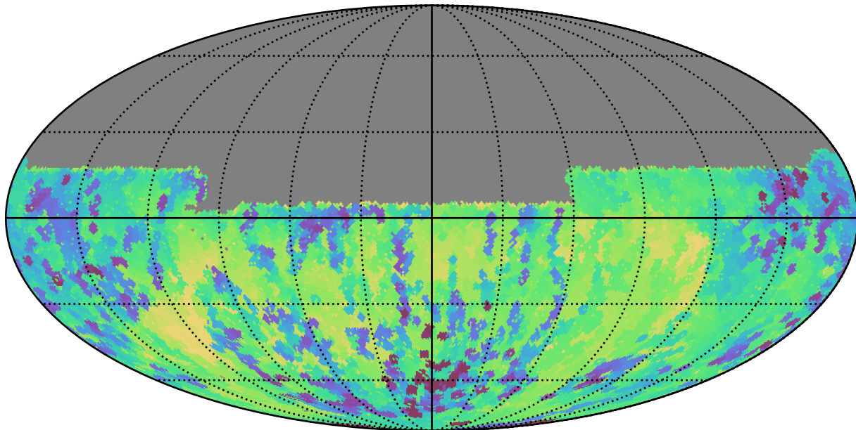
weather_cloudso1v3.4_10yrs Yr 1 y band: Min skyBrightness
