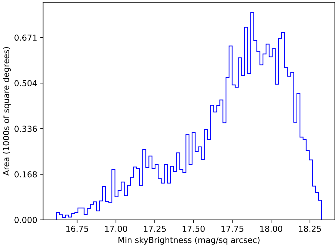
weather_cloudso1v3.4_10yrs Yr 1 y band: Min skyBrightness
