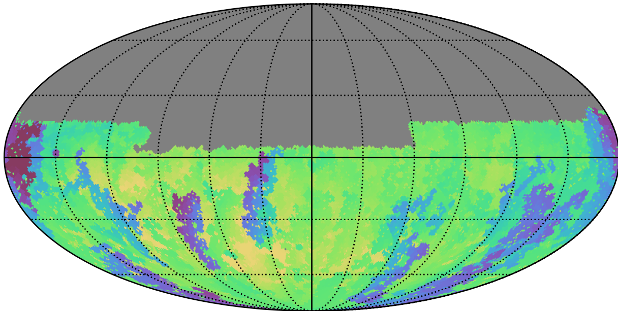
weather_cloudso1v3.4_10yrs Yr 1 u band: Min skyBrightness
